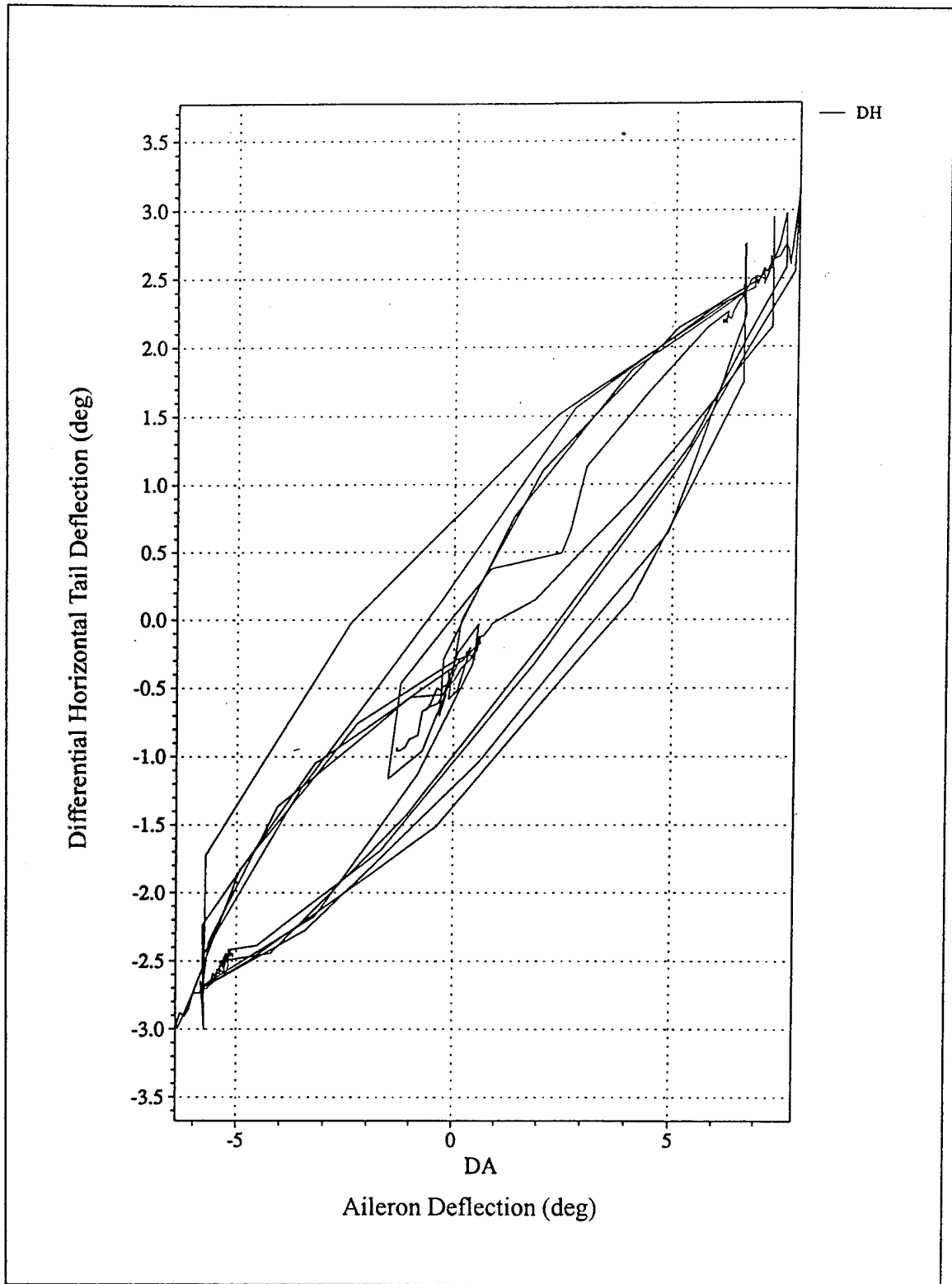
Figure 2.7. High Correlation between two Control Surface Inputs.
